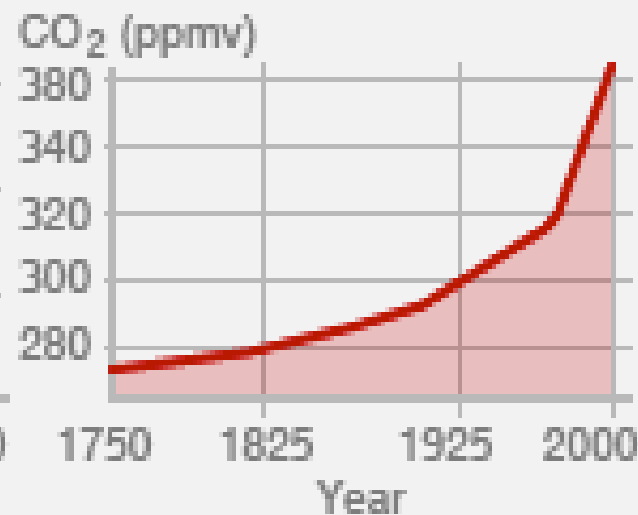
CO 2 CONCENTRATION
